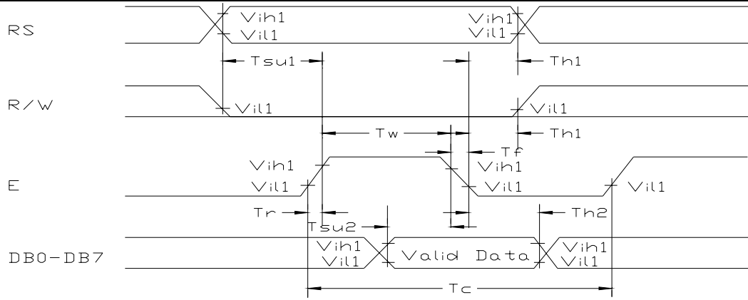
(2) Read mode(Reading data fromST7066U to MCU)
